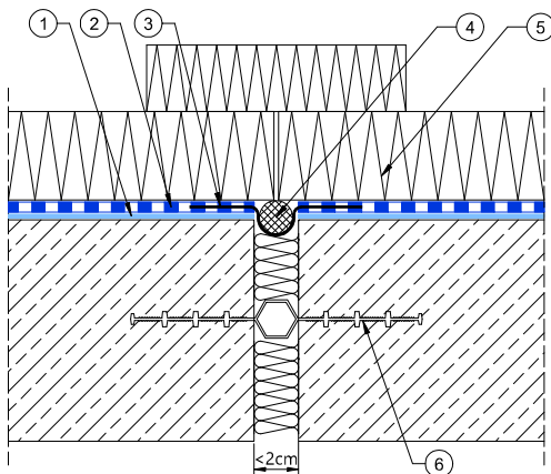
Expansion joint detail – waterproofing
