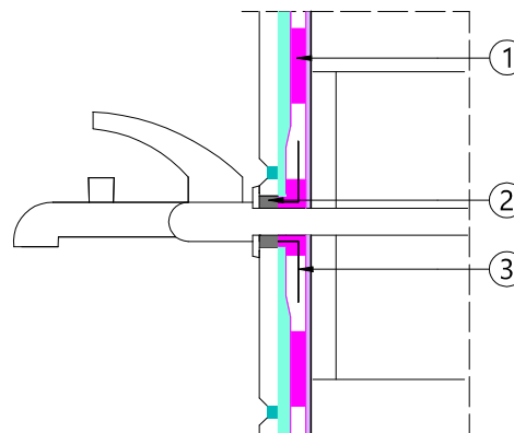
Detail of pipe passage through wall
