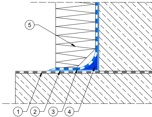
Detail of footing and foundation wall connection-waterproofing
