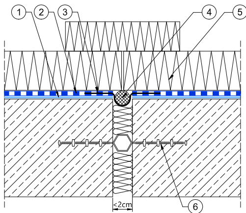
Expansion joint detail - waterproofing insulation
